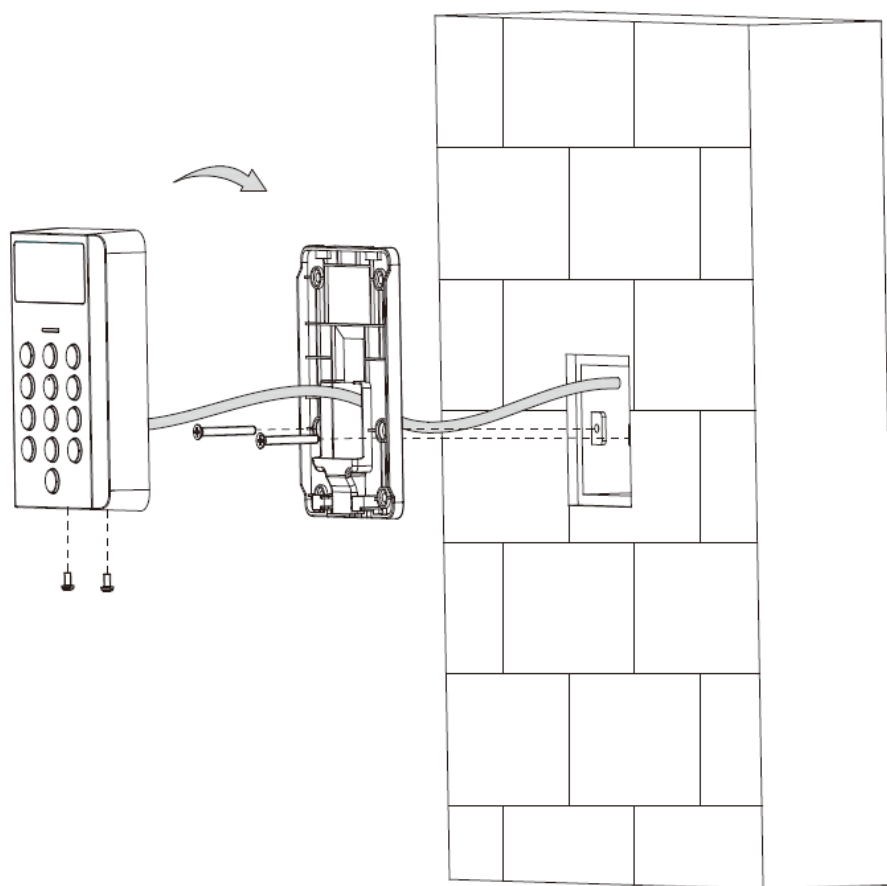
Figure 3-8 86-box mount
