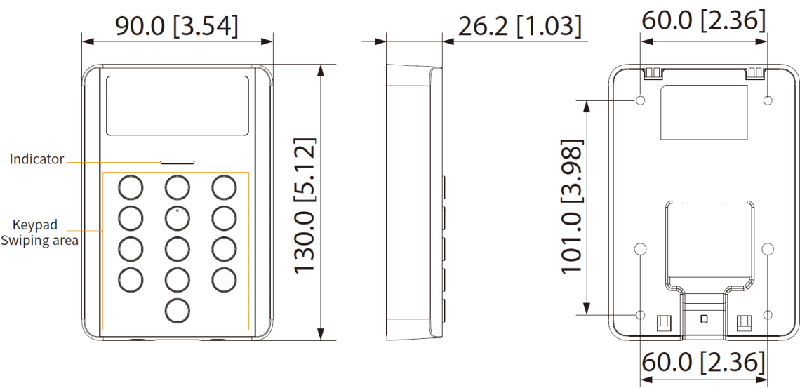
Figure 2-1 Appearance and dimensions (unit: mm [inch])
