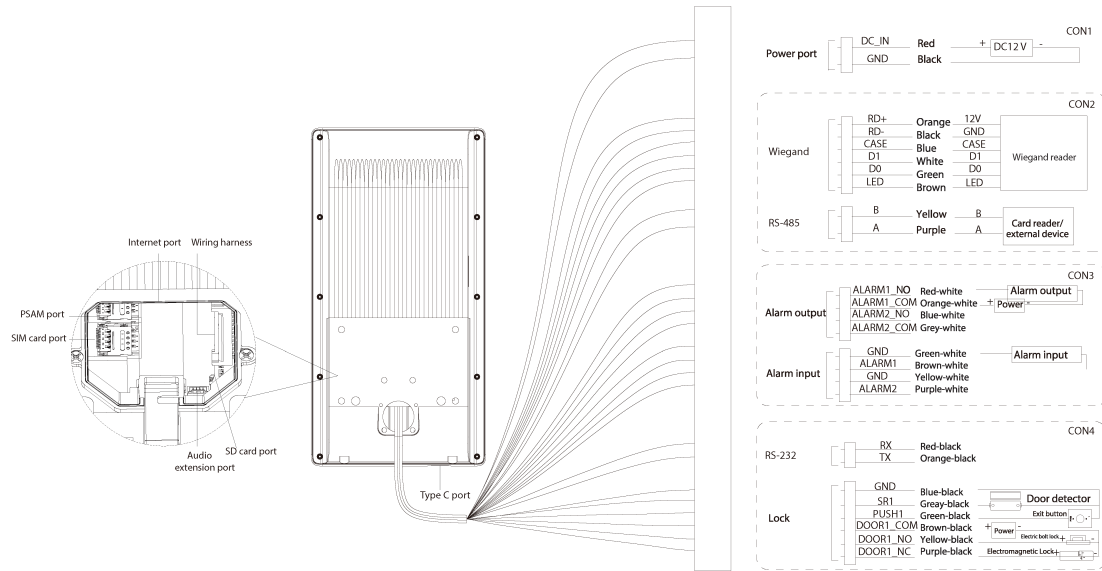
Figure 2-1 Cable connections
