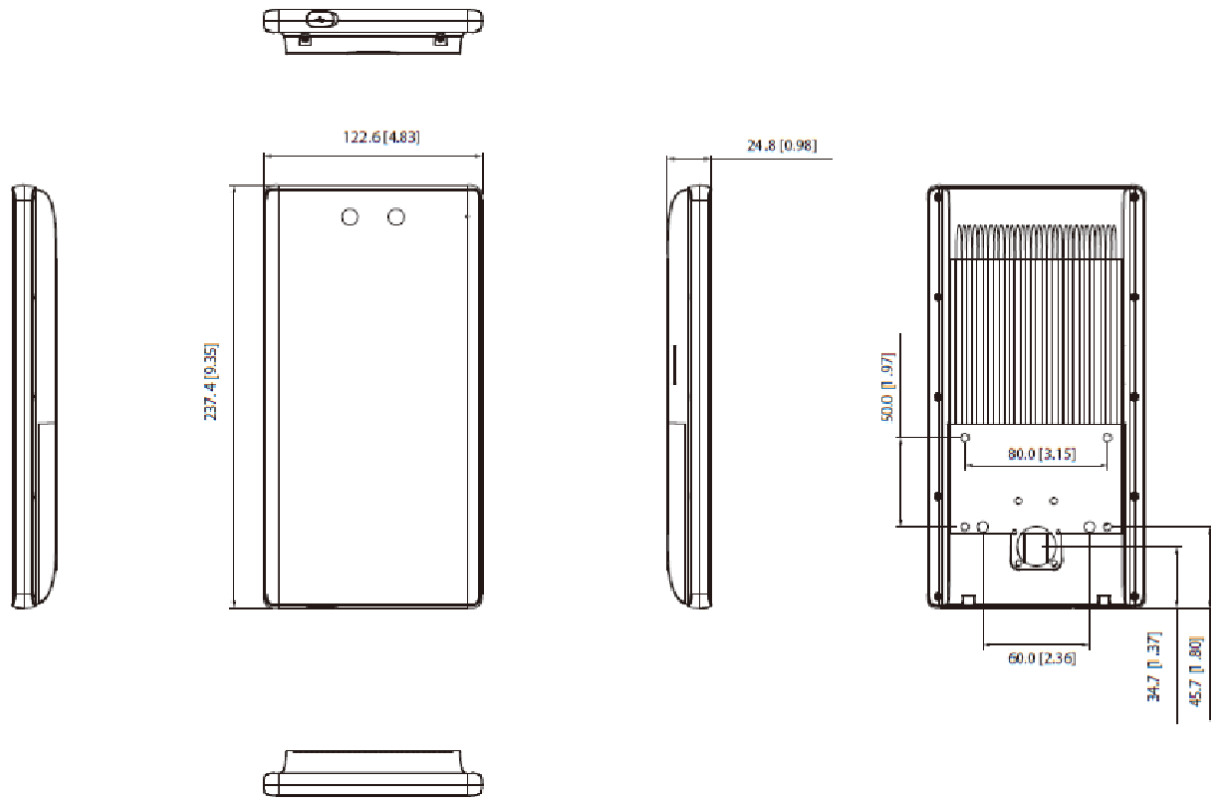
Figure 1-1 Structure (Unit: mm [inch])
